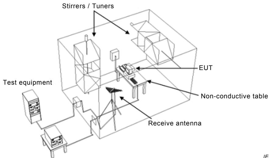
Figure I.4 – Overview of the reverberation chamber for radiated emission measurement
